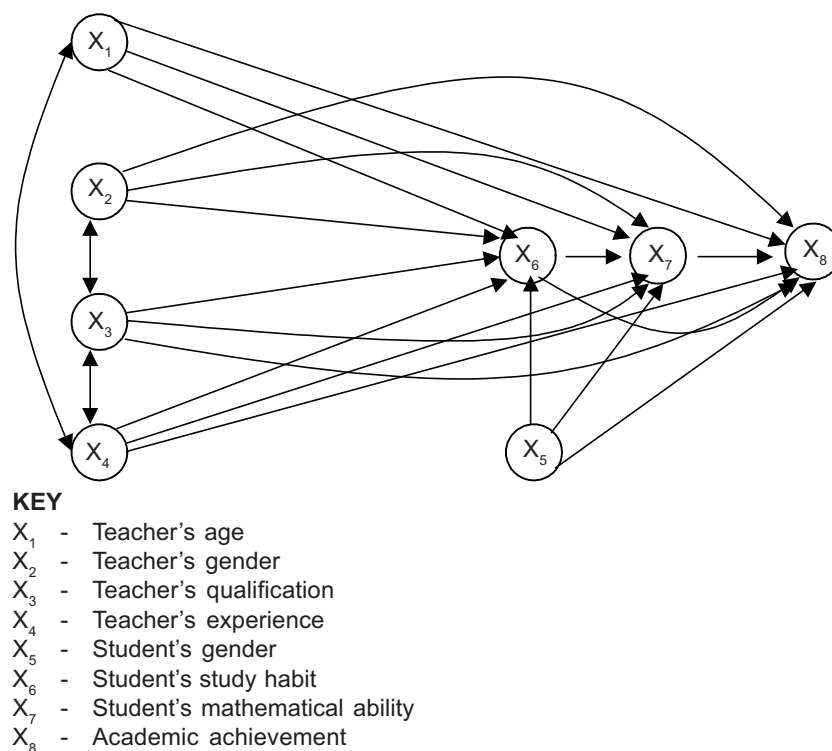
FIGURE 1. Hypothesized causal model
