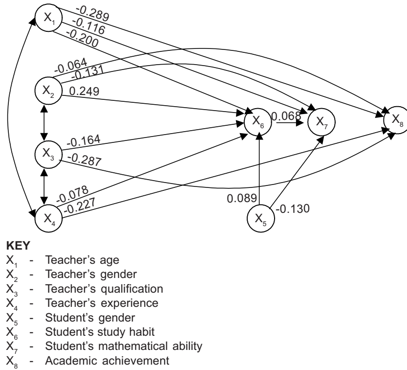
FIGURE 2. Structural equations
